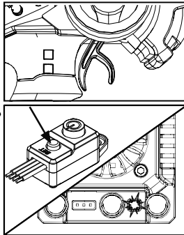
2. TX full throttle - press set button (2 Green flashes)
